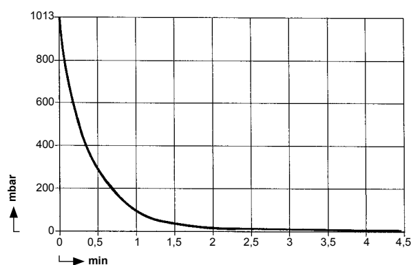
PUMP DOWN TIME FOR 20 LITER VESSEL
