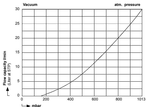
FLOW CAPACITY
