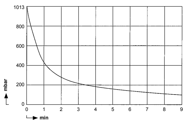
PUMP DOWN TIME FOR 5 LITER VESSEL
